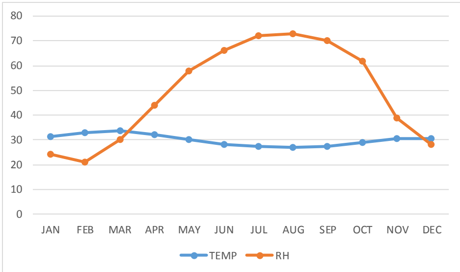
Figure 2. Monthly mean temperature and relative humidity of the study area
