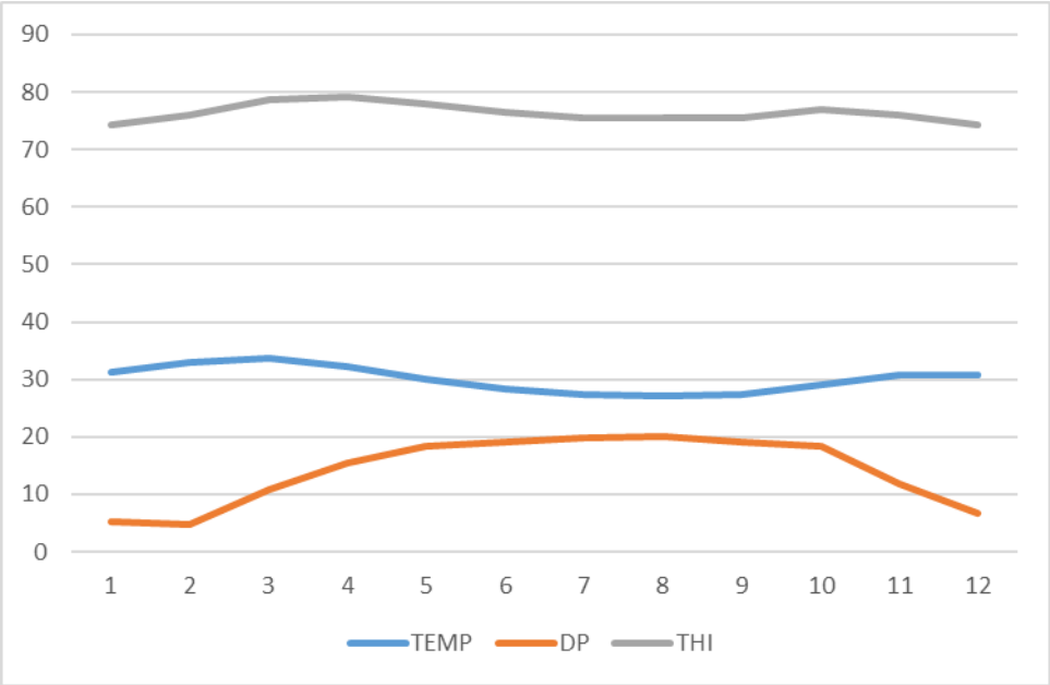
Figure 1. Monthly Temperature (TEMP), Dew Point temperature (DP) and THI (in °F)
